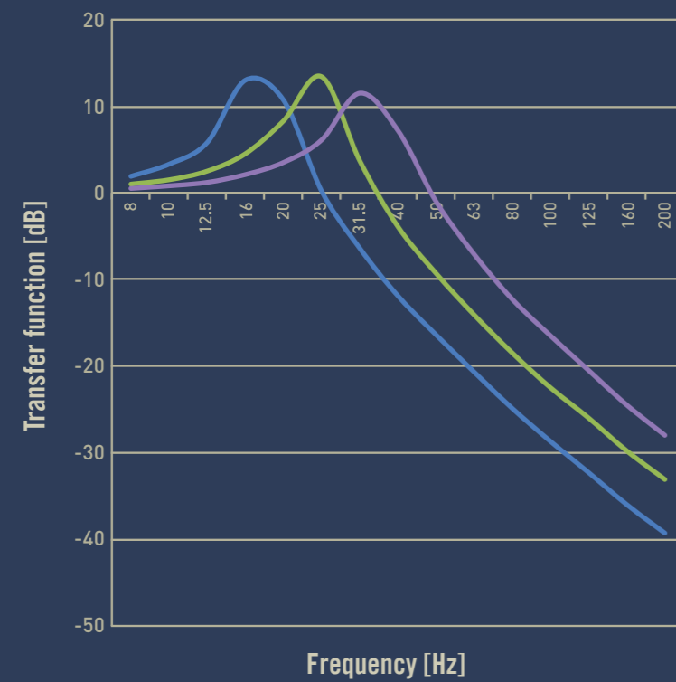
LVT TRANSFER FUNCTION
